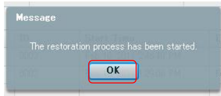
Figure 27 Managing Disks
