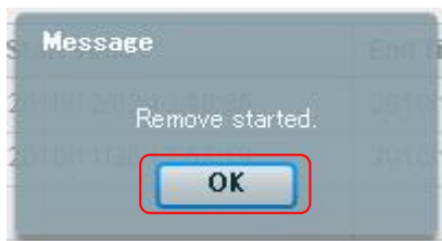
Figure 35 Managing Disks
