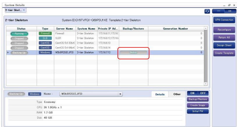
Figure 36 Managing Disks
