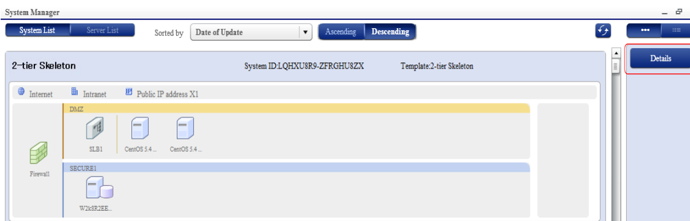
Figure 15 Managing Disks
