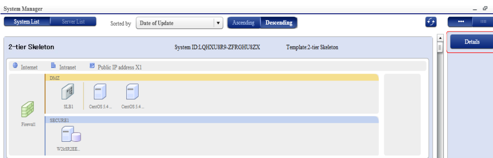
Figure 1 Managing Disks
