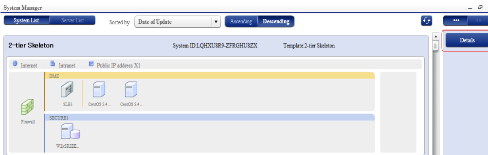
Figure 8 Managing Disks
