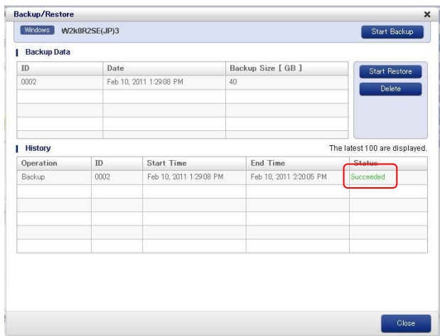
Figure 37 Managing Disks
