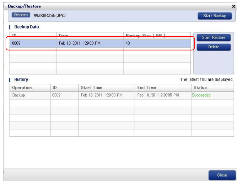
Figure 24 Managing Disks
