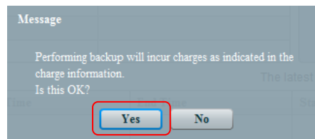
Figure 4 Managing Disks
