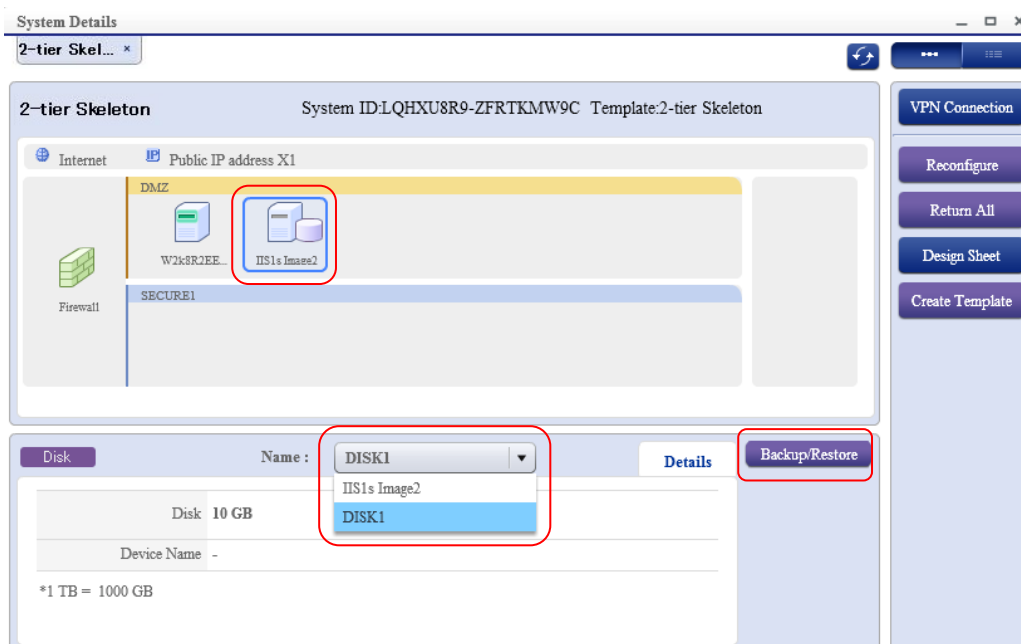
Figure 23 Managing Disks
