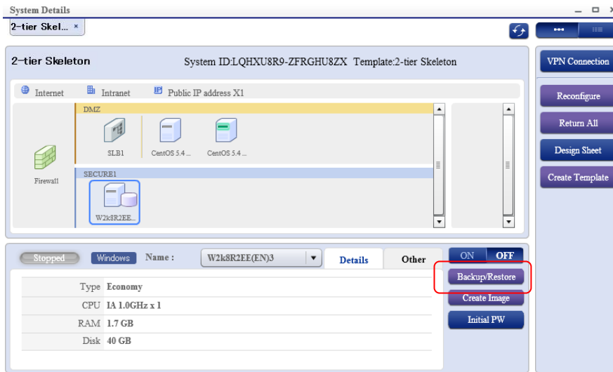
Figure 16 Managing Disks
