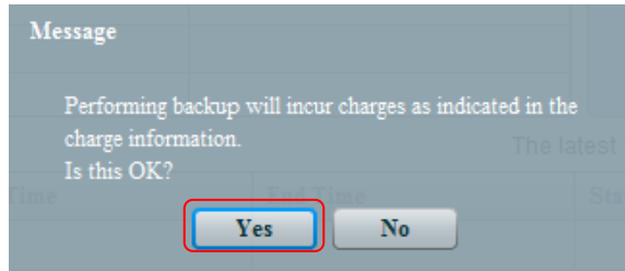
Figure 11 Managing Disks
