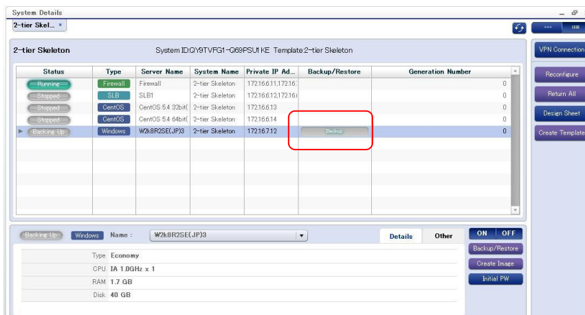
Figure 6 Managing Disks
