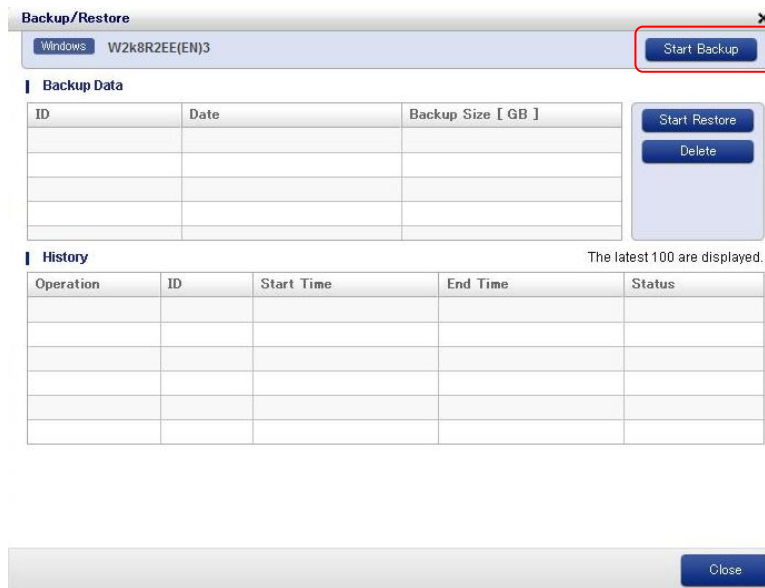
Figure 3 Managing Disks
